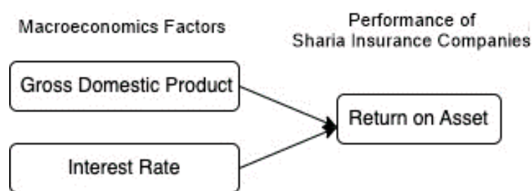
Figure 1. Research variables
