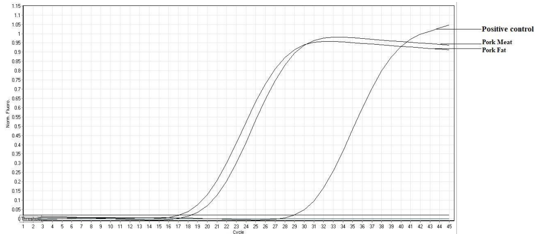
Figure 3. Amplification Curves of Raw Pork Meat and Pork Fat
