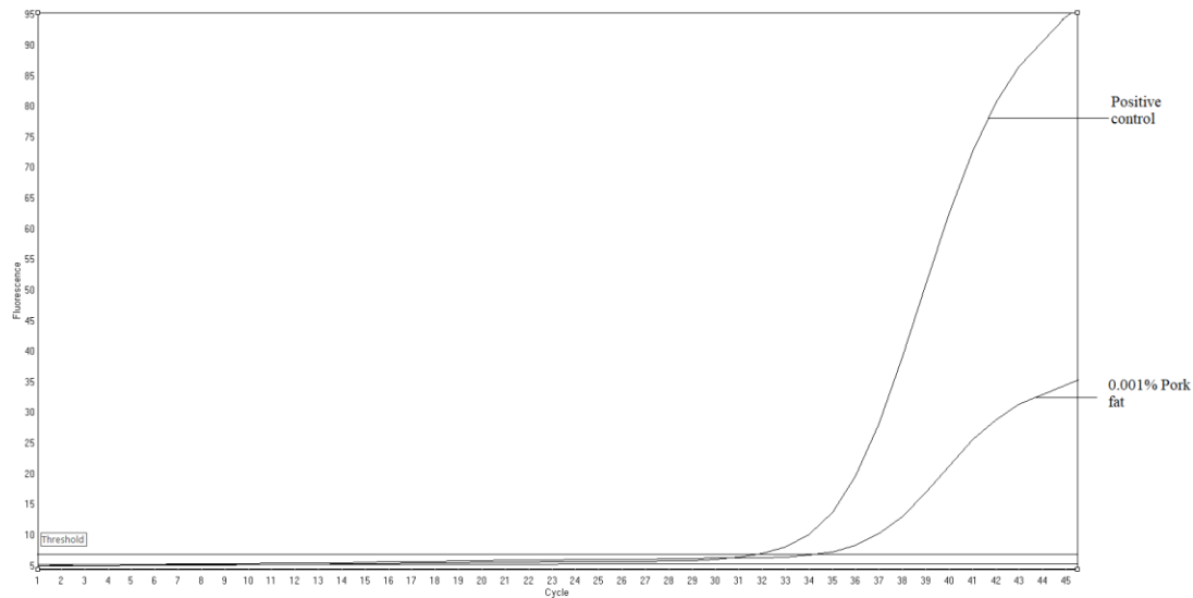
Figure 6. Amplification Curve Showing 0.001% Pork Contamination.
