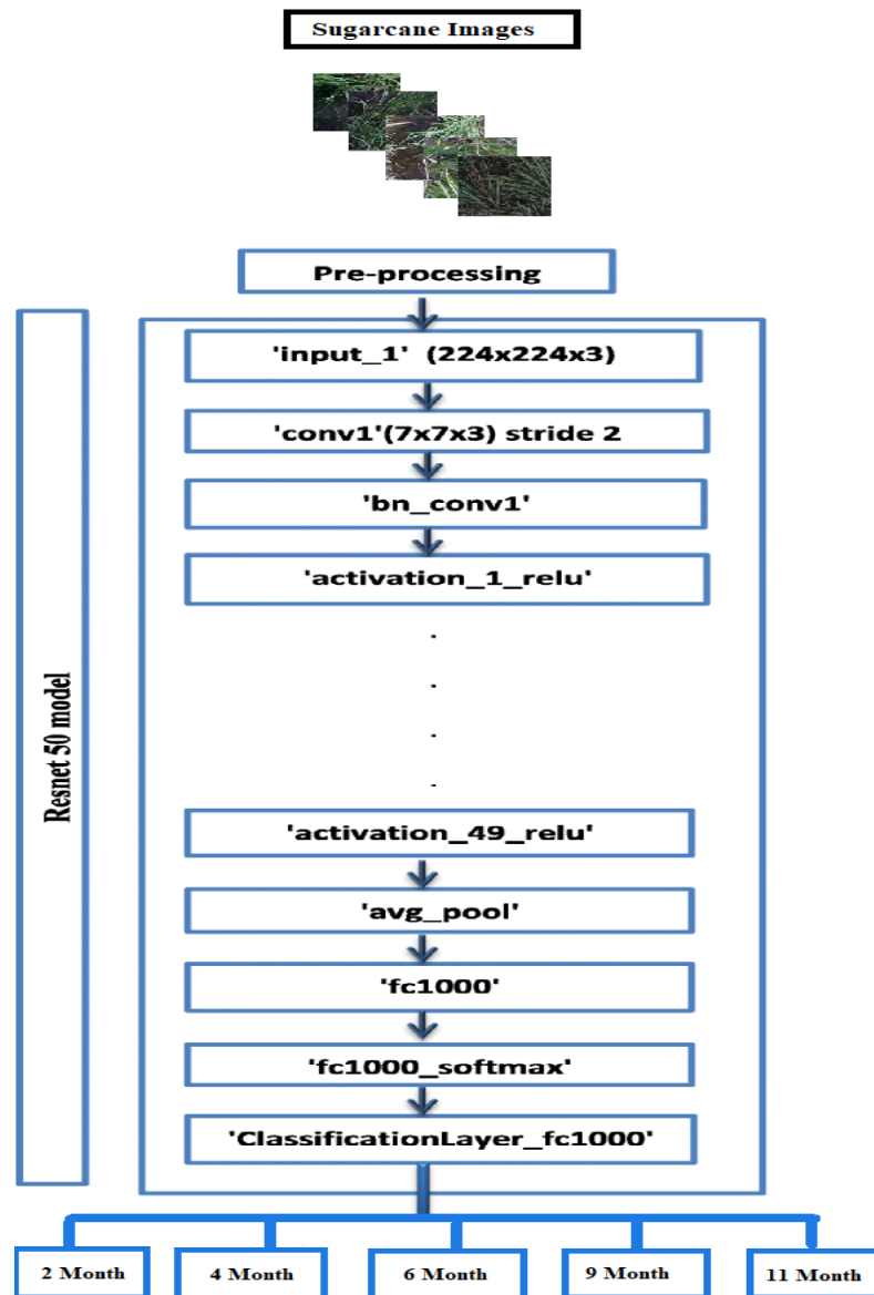
Figure 2. Resnet50 Architecture
